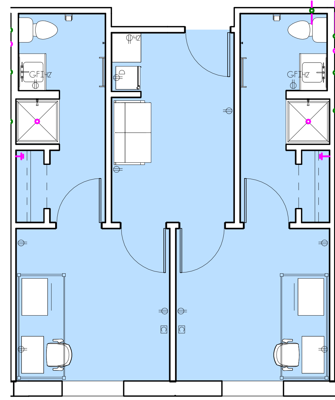
3 ENLARGED FURNITURE PLAN - 2BR / 2B 1/4" = 1'-0"
